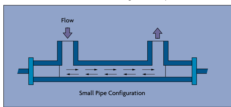
Figure 4-10: Axial Flowmeter
