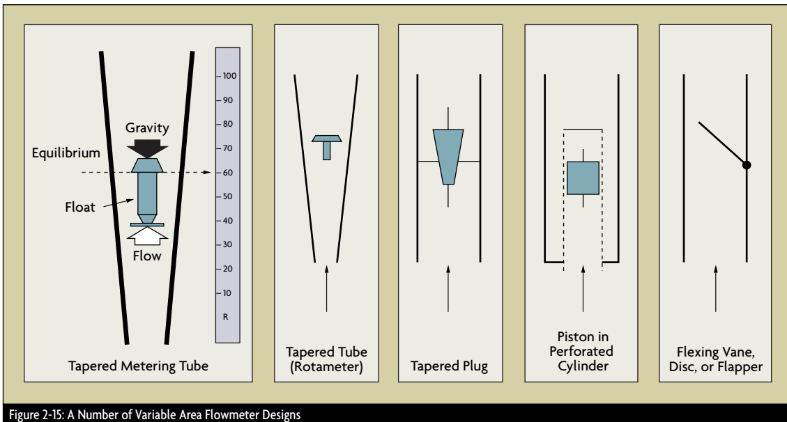
Figure 2-15: A Number of Variable Area Flowmeter Designs
