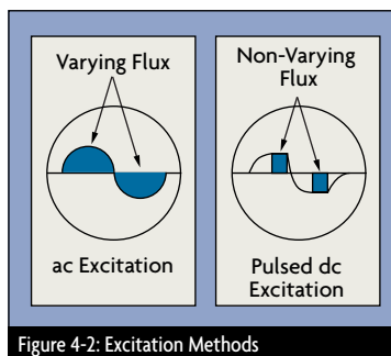
Figure 4-2: Excitation Methods
