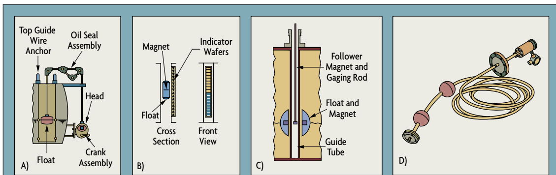
Figure 7-12: Continuous Float Level Detectors
